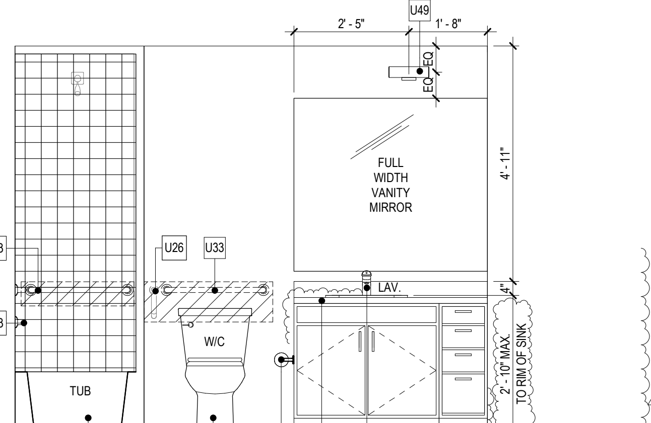
UNIT C-2a ACC. BATHROOM ELEV.
