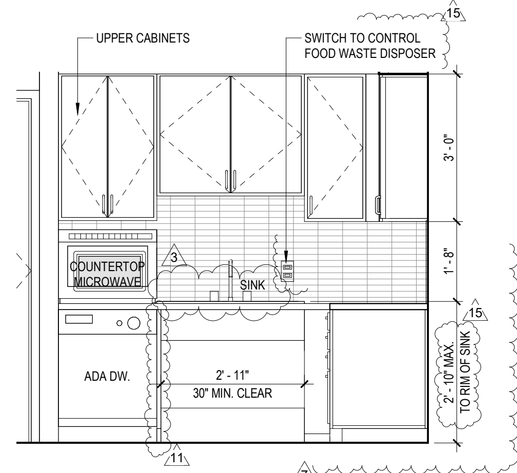
UNIT C-2a ACC. KITCHEN ELEV.
