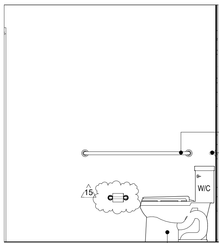
UNIT C-2a ACC. BATHROOM ELEV.
