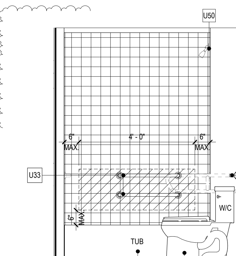
UNIT C-2a ACC. BATHROOM ELEV.
