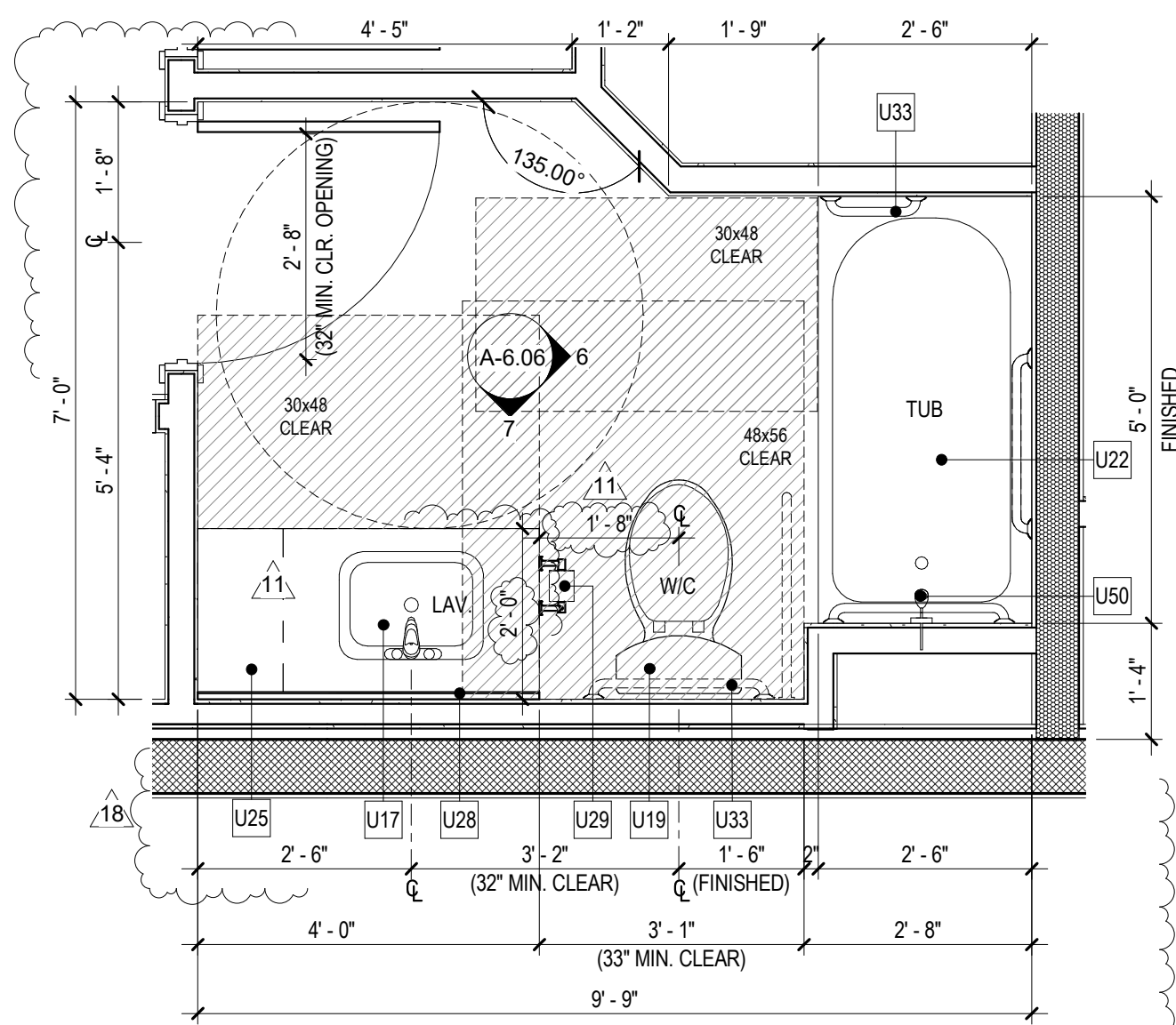
UNIT C-2a ACC. BATHROOM
