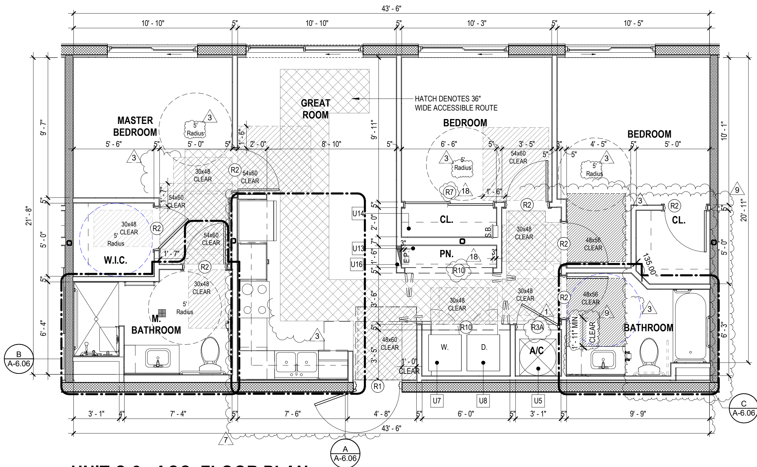
UNIT C-2a ACC. FLOOR PLAN
