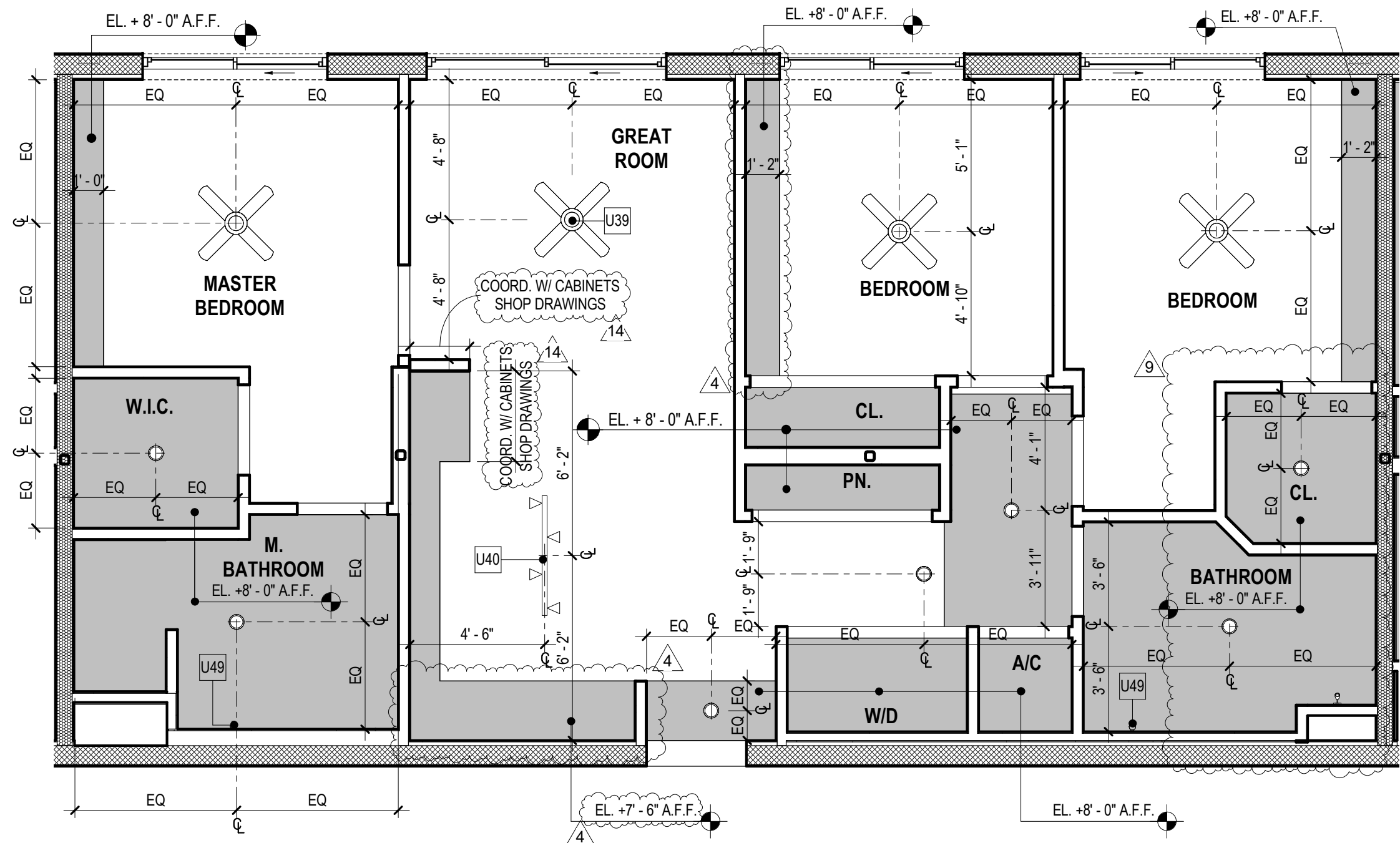
UNIT C-2a ACC. RCP
