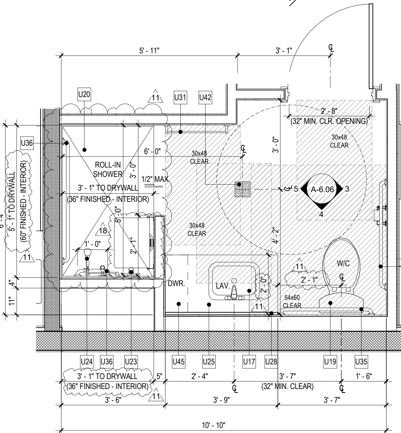
UNIT C-2a ACC. M. BATHROOM
