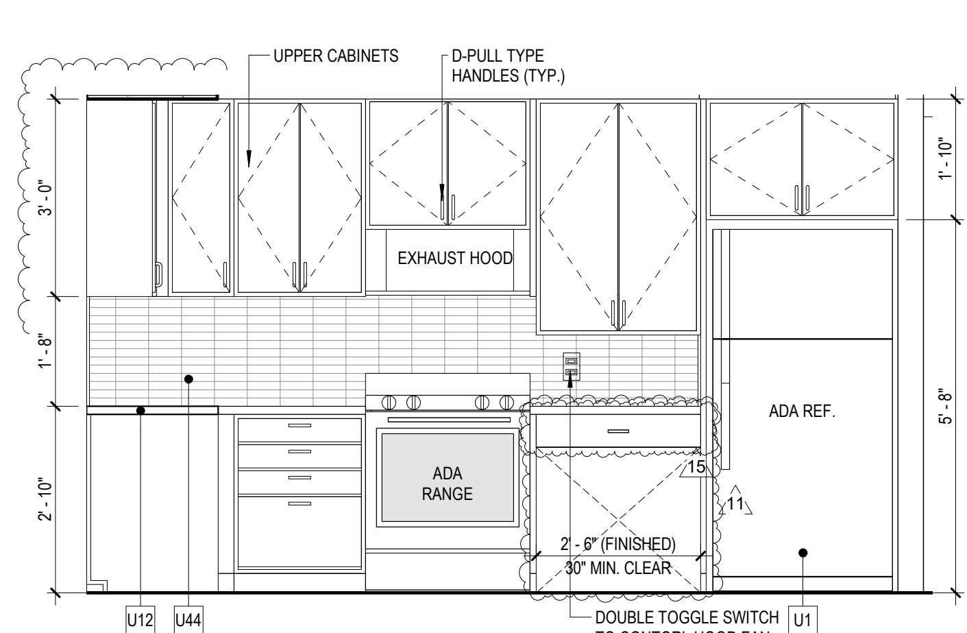
UNIT C-2a ACC. KITCHEN ELEV.
