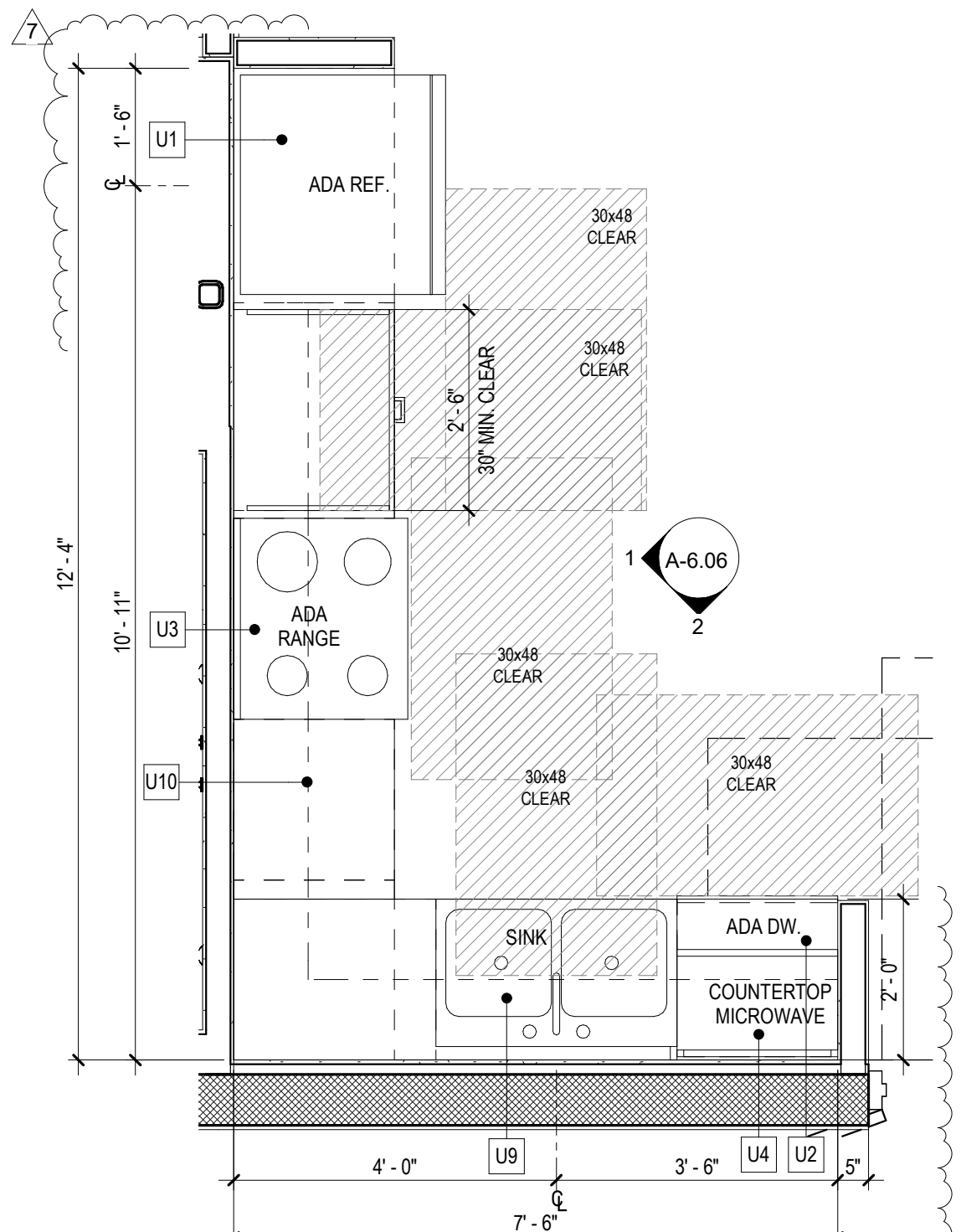
UNIT C-2a ACC. - KITCHEN
